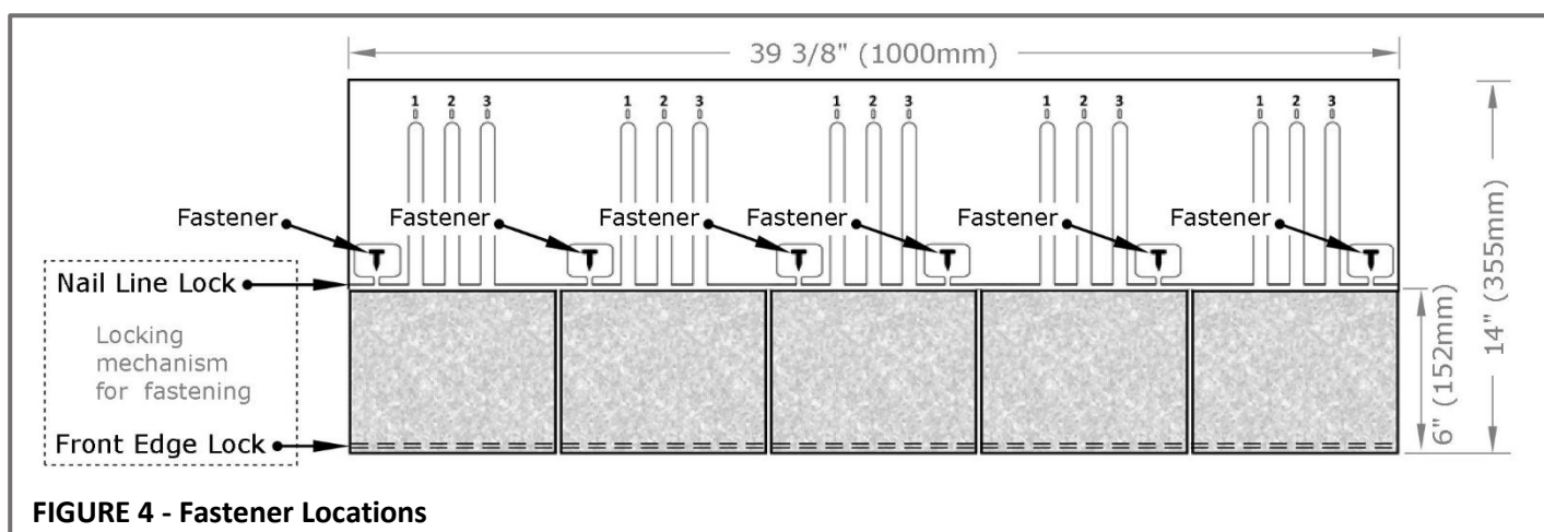
FIGURE 3 - Fastening
