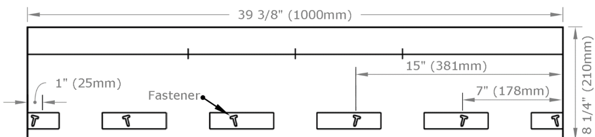
FIGURE 6 - Starter
