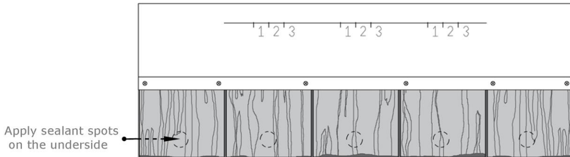
FIGURE 5 - Sealant Spots
