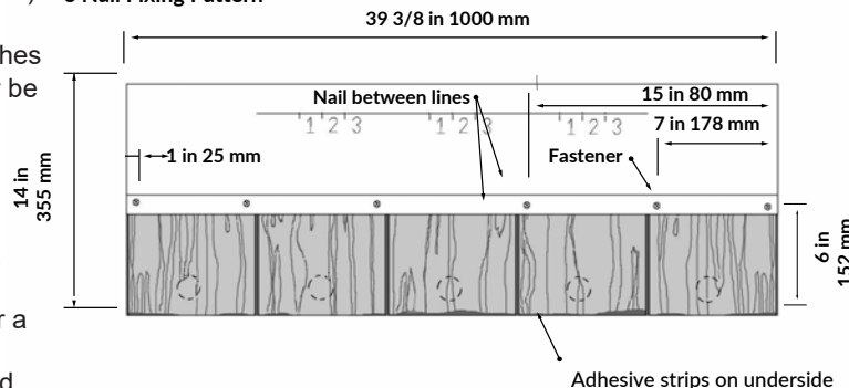
6 Nail Fixing Pattern
